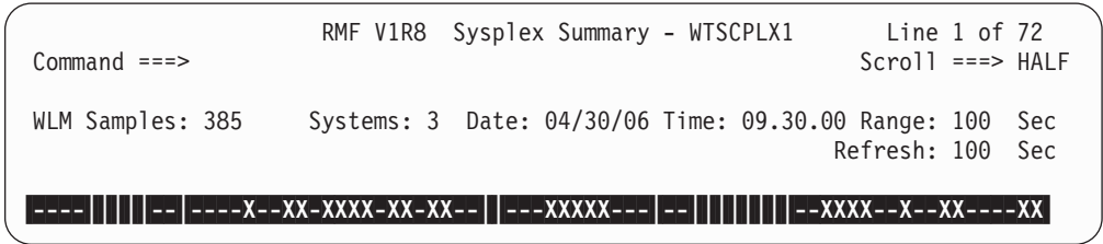
Figure 14. Monitor III Sysplex Summary Report - GO Mode
